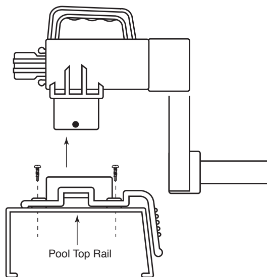
SOCKET STYLE ASSEMBLY
